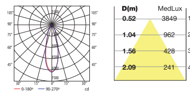
LED 3000lm 24° 3000K
