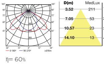
TL5 G5 1x39W double parabolic
