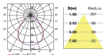
LED 18W Blanco neutro / Neutral white
