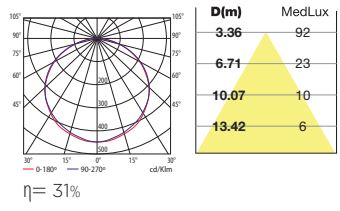
TL5 G5 1x54W polycarbonate
