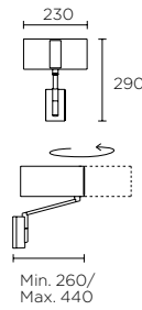
05-2817-81-14 1 X E-27 MAX. 60W ESF. Ø45 | Ø= 70 MM L= 130 MM HALOGEN - FLUORESCENT - LED
