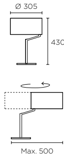
10-2817-81-14 1 X E-27 MAX. 60W ESF. Ø45 | Ø= 70 MM L= 130 MM HALOGEN - FLUORESCENT - LED
