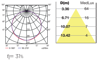
TL5 G5 1x39W polycarbonate
