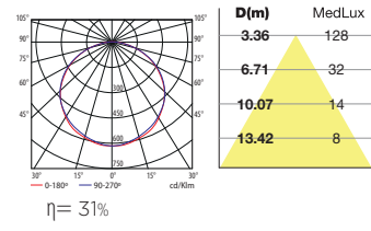
TL5 G5 1x80W polycarbonate
