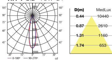
HIT-T G12 70W 24°
