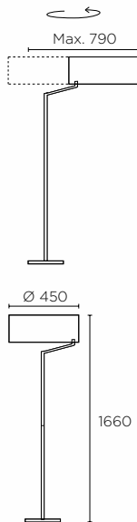
25-2817-81-14 1 X E-27 MAX. 150W | L= 250 MM HALOGEN - FLUORESCENT - LED
