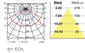
TL5 G5 1x80W double parabolic
