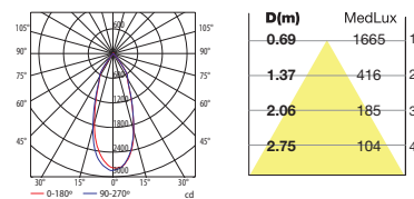
LED 2000lm 36° 3000K
