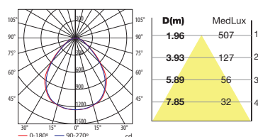
LED 26W Blanco neutro / Neutral white
