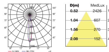
LED 2000lm 24° 3000K
