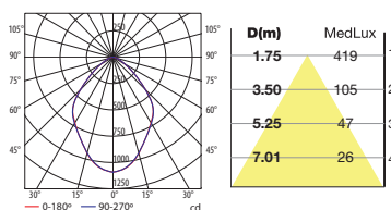
LED 18W Blanco neutro / Neutral white
