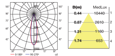
HIT-T G12 70W 24°
