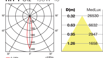
HIT-T G12 150W 10°
