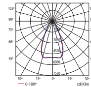
HIT-T G12 70W 38°
