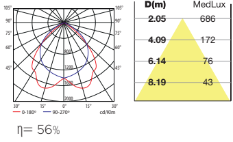
TL5 G5 2x39W double parabolic
