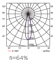
HIT-T G12 70W 24°
