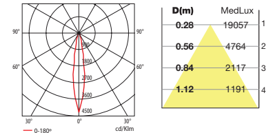
HIT-T G12 70W 10°
