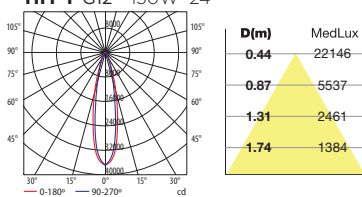
HIT-T G12 150W 24°
