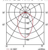
HIT-DE RX7s 70W
