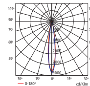
HIT-T G12 70W 12°
