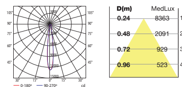
LED 2000lm 15° 3000K
