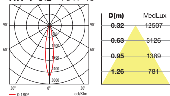
HIT-T G12 70W 10°
