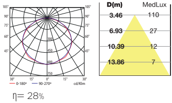
TL5 G5 2x39W polycarbonate
