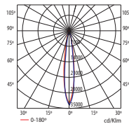
HIT-T G12 70W 10°
