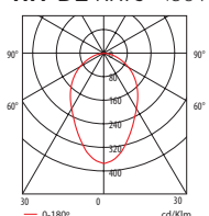
HIT-DE RX7s 150W
