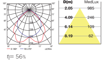
TL5 G5 2x54W double parabolic
