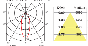
HIT-T G12 150W 45°
