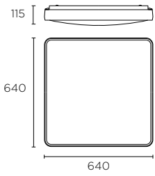
15-4688-14-M1 | 15-4688-S2-M1 3 X 2G11 55W
