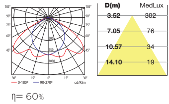
TL5 G5 1x54W double parabolic
