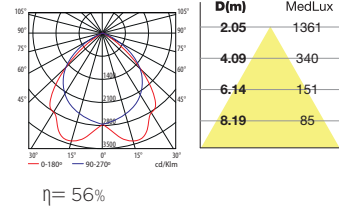
TL5 G5 2x80W double parabolic
