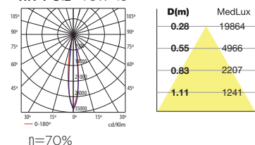
HIT-T G12 70W 10°
