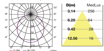
15-2920-52-M1 LED Blanco neutro / Neutral white
