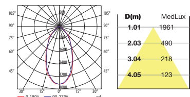
HIT-TC G8.5 70W
