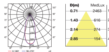
LED 3000lm 36° 3000K
